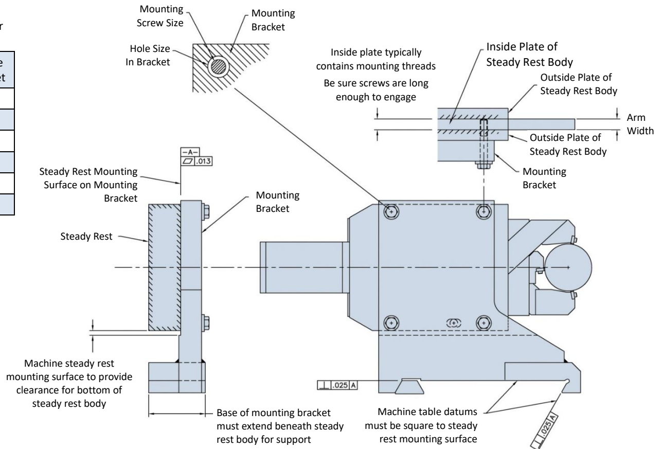
Over-Sized Holes Recommended For Mounting Screws
